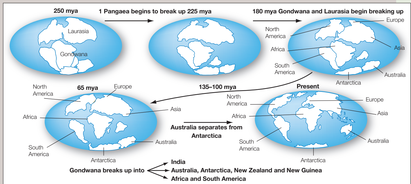
Pangaea and the separation of continents
